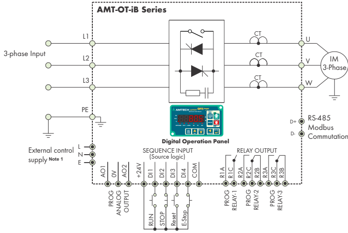
In-line configuration
